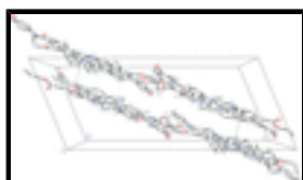
Fig. 2. The crystal packing of the title compound, viewed along the b axis. Dashed lines indicate hydrogen bonds. H atoms not involved in the hydrogen bond interactions have been omitted for clarity.
