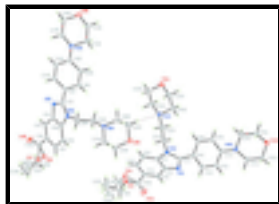
Fig. 1. The asymmetric unit of the title compound, showing 50% probability displacement ellipsoids and the atom-numbering scheme. Hydrogen atoms are shown as spheres of arbitrary radius.
